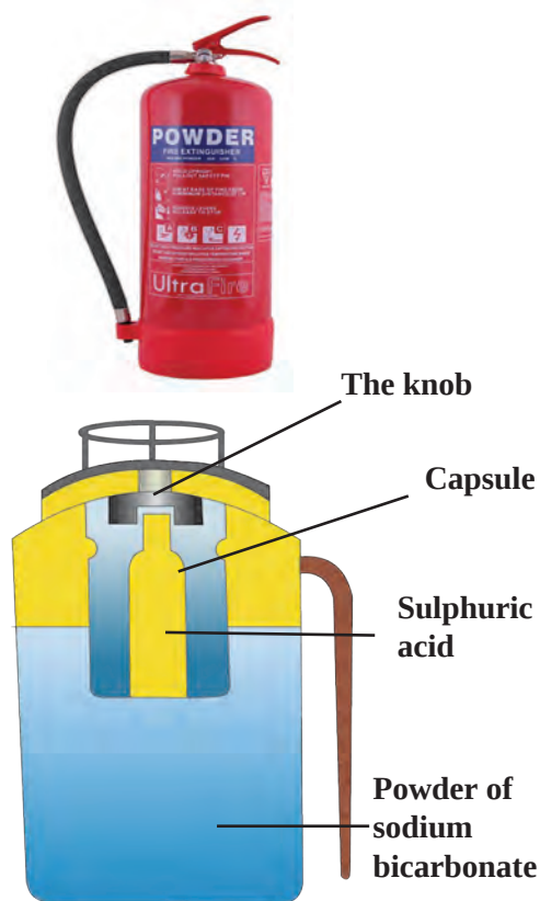
13.12 Internal structure of fire extinguisher
