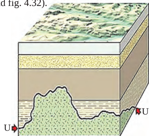
Fig. 4.31: Nonconformity
