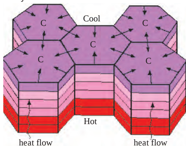
Fig. 4.25 : Columnar joints
