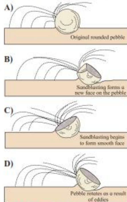
Fig. 3.17 : Formation of a typical ventifact
