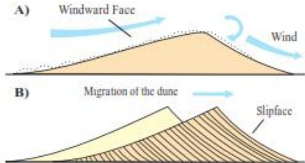
Fig. 3.23 : Migration of dunes
