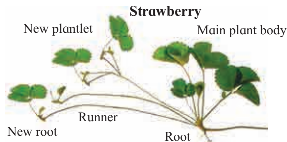
Fig. 9.23 Runner
