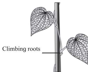
Fig. 9.11 Climbing roots
