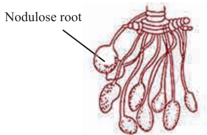
Fig. 9.8 Nodulose root
