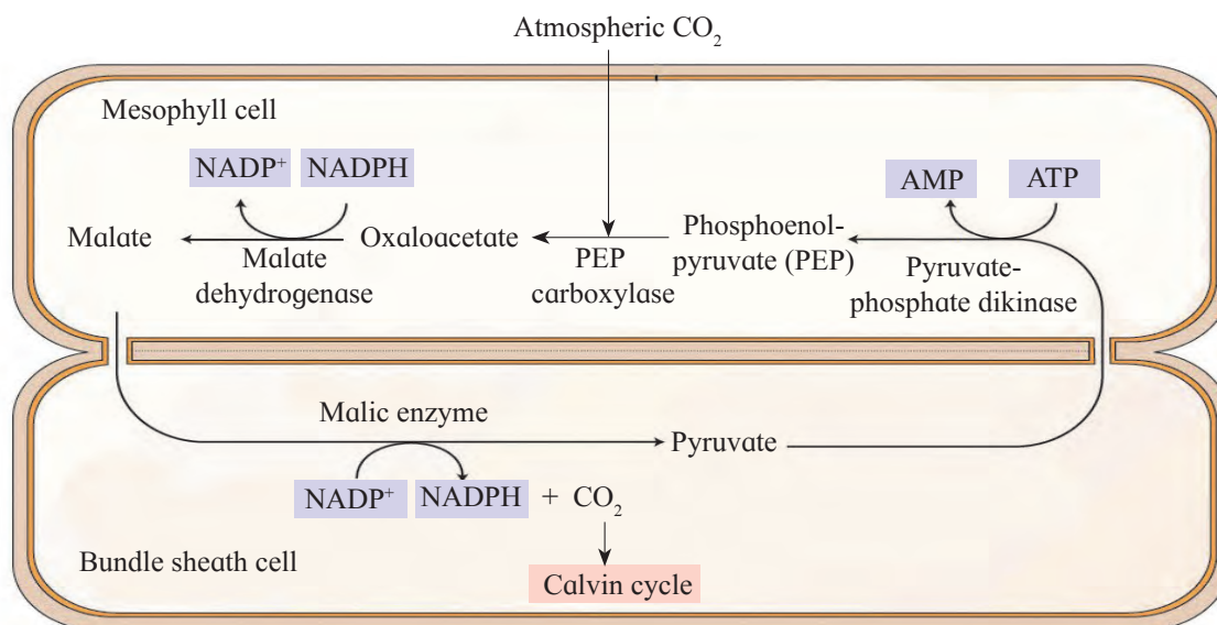
Fig. 12.13 C_4 Pathway
