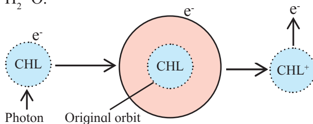
Fig. 12.5 Photoexcitation of chlorophyll-a
